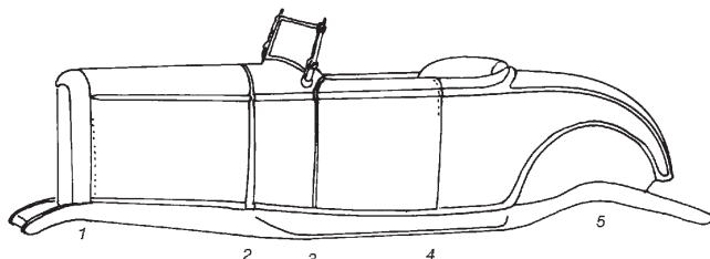
C. Grille and rear of body are high (reference points 1 & 5). Doors overlap quarter at top. Wide gap at lower rear of hood tapering to normal at top. Lower front hood overlaps grille, normal gap at top.
