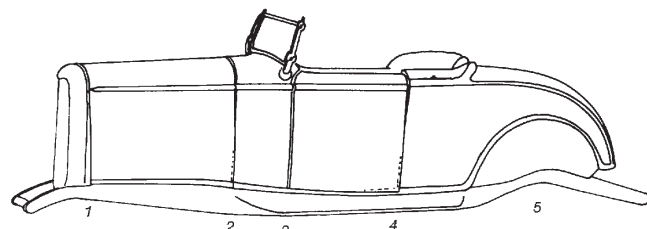
D. Body is too high at front of cowl (reference 2) Doors overlaps and drops at quarter, Grille is pulled back. Back lower corner of hood overlaps cowl. Normal gap top front of hood tapering to wide at bottom.
