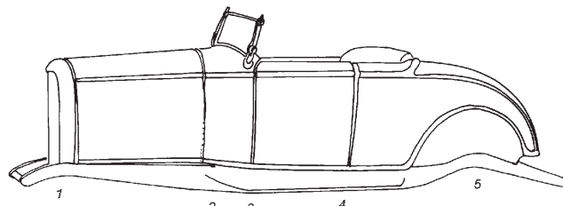
B. Body is too high at middle (reference points 2,3, and 4). Wide gap at top of door tapering to normal at bottom. Normal gap at hood top front tapering to wide at bottom. Rear bottom of hood overlaps cowl, normal gap at top.
